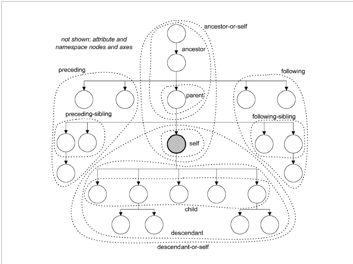
XPath Achsen, Quelle Crane Softwrights, 2001
